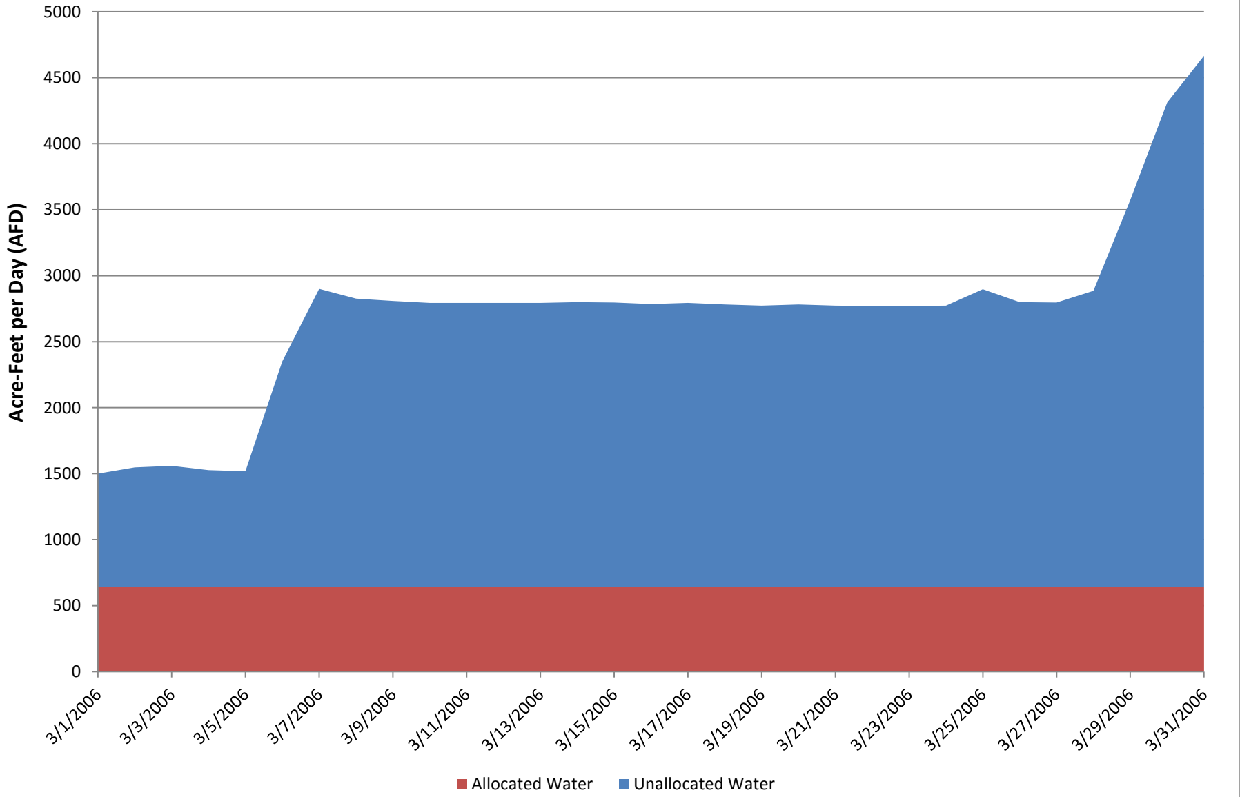
Figure H-83: Daily Unallocated Water Calculation Downstream of Camanche Reservoir - March 2006 hydrology (2040 diversion assumptions)
