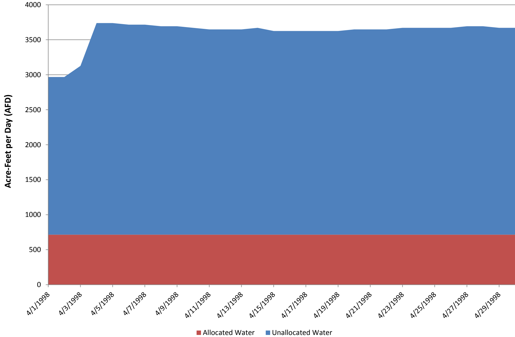
Figure H-60: Daily Unallocated Water Calculation Downstream of Camanche Reservoir - April 1998 hydrology (2040 diversion assumptions)
